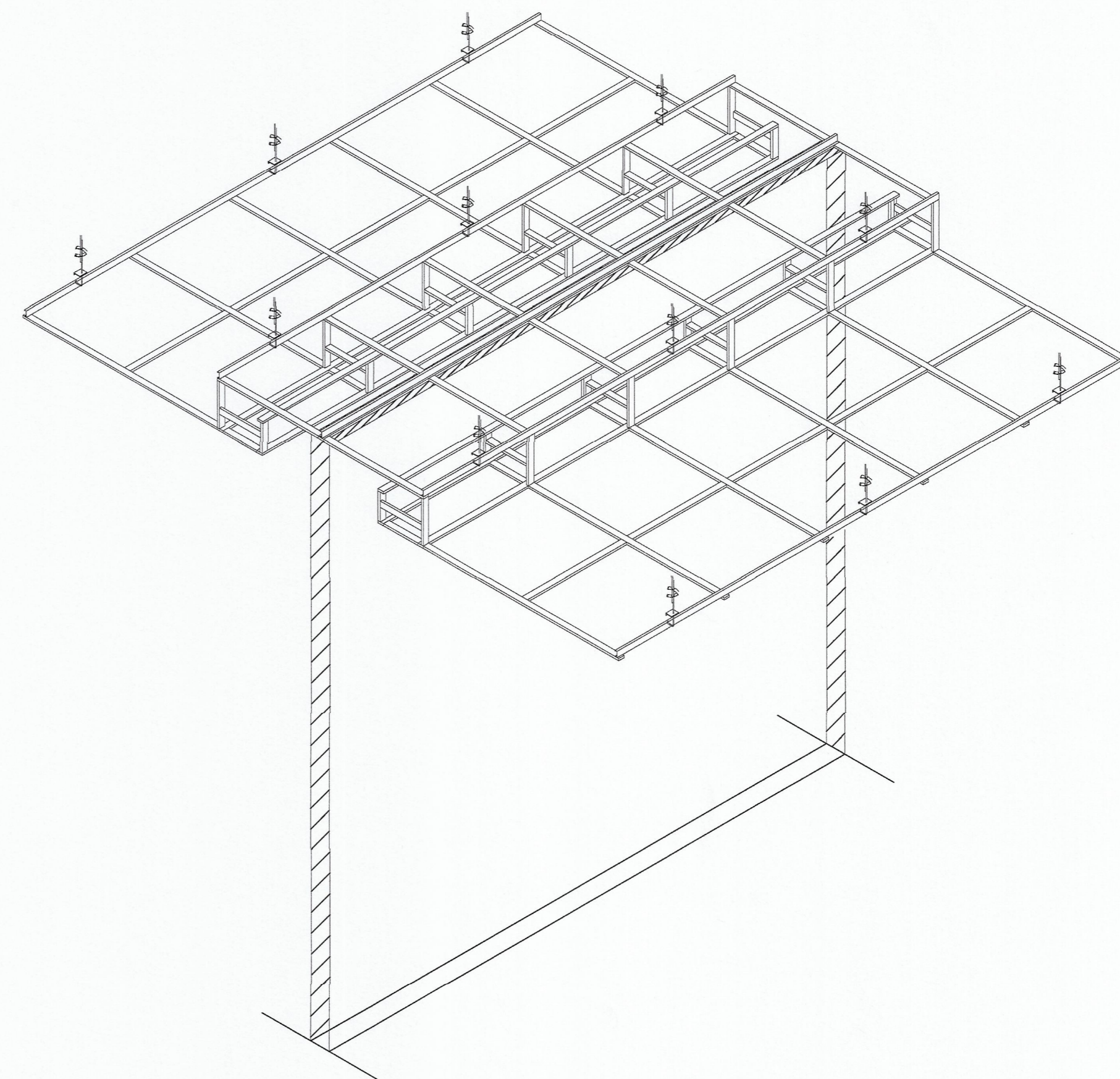
ISOMETRIC CEILING GI-FURRING PLAN SCALE NOT TO SCALE
