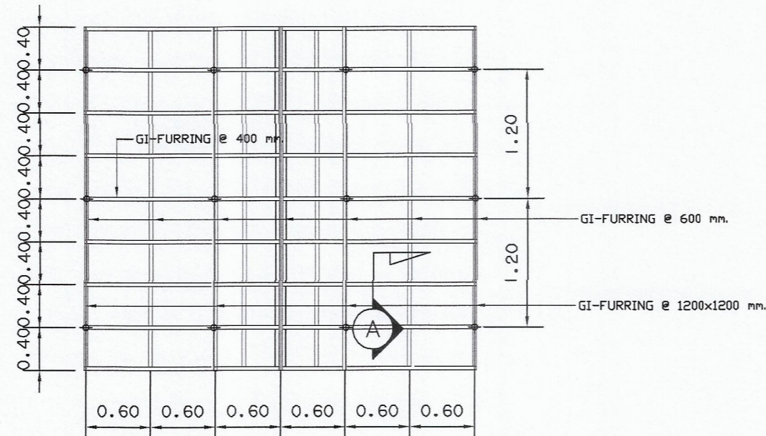
CEILING GI-FURRING PLAN SCALE 1 : 20
