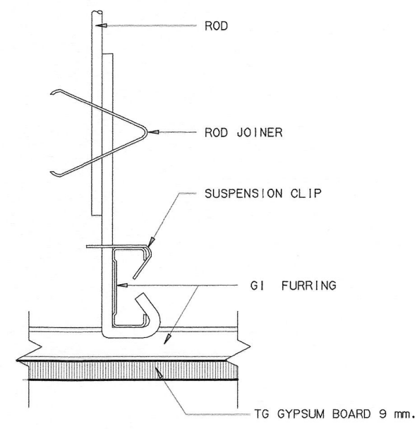
SECTION N.T.S Typical detail
