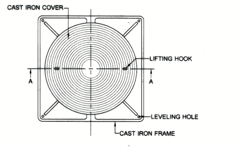
MANHOLE COVER DETAIL
