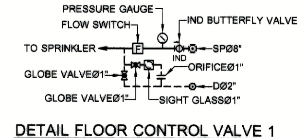
DETAIL FLOOR CONTROL VALVE 1
