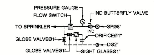
DETAIL FLOOR CONTROL VALVE 1
