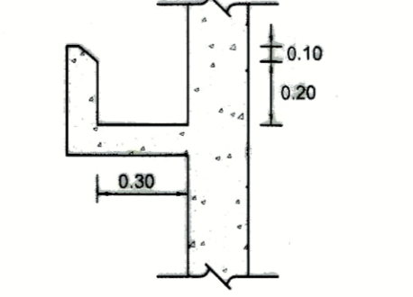
DETAIL OVERFLOW WEIR
